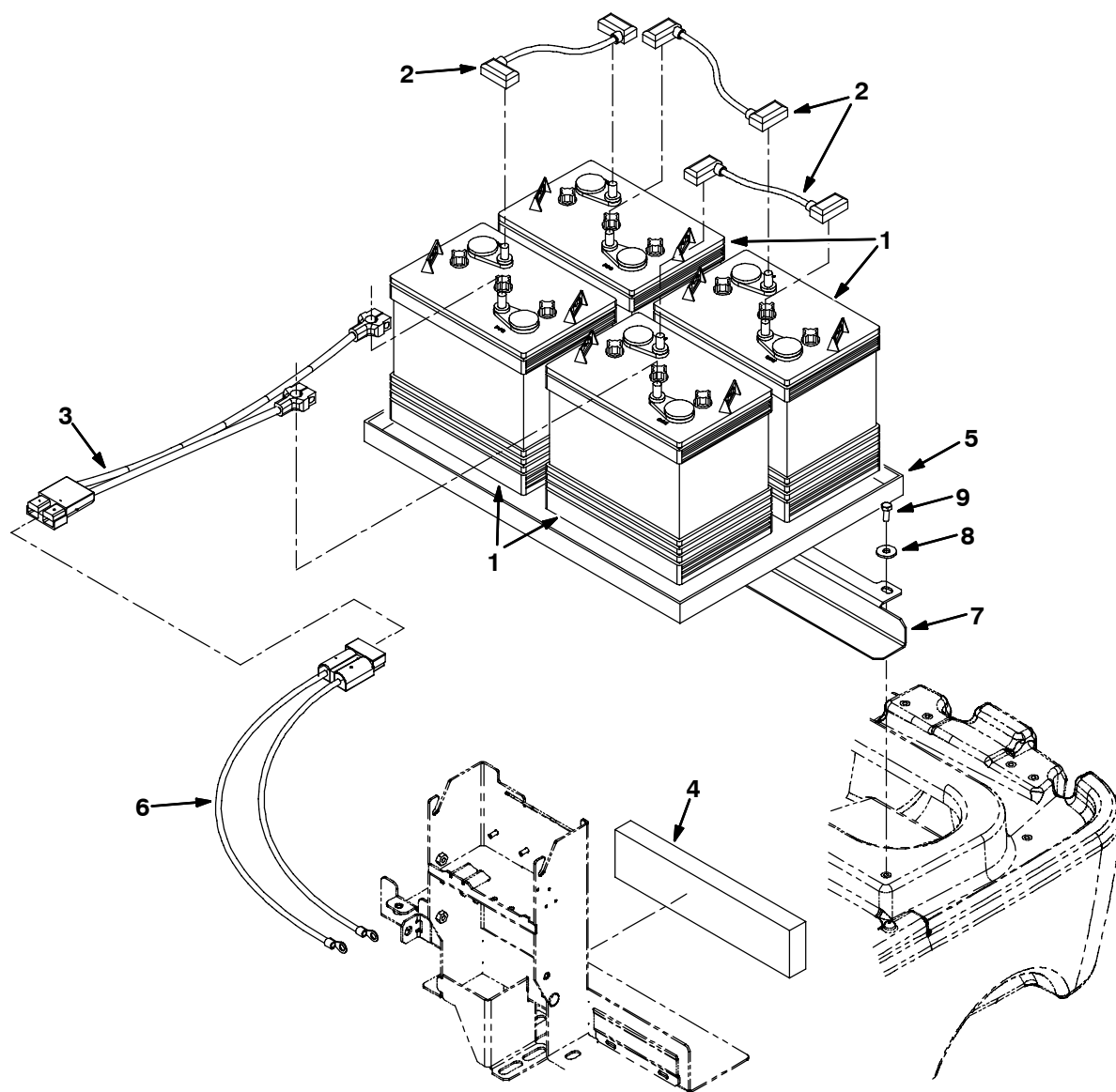
Fig. 6 - Battery and Charger Group 255Ah/5H
