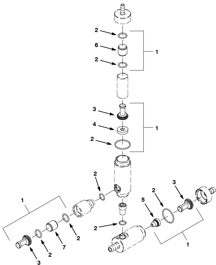
Fig. 1 - FaST Injector Assembly Breakdown, 9003909
