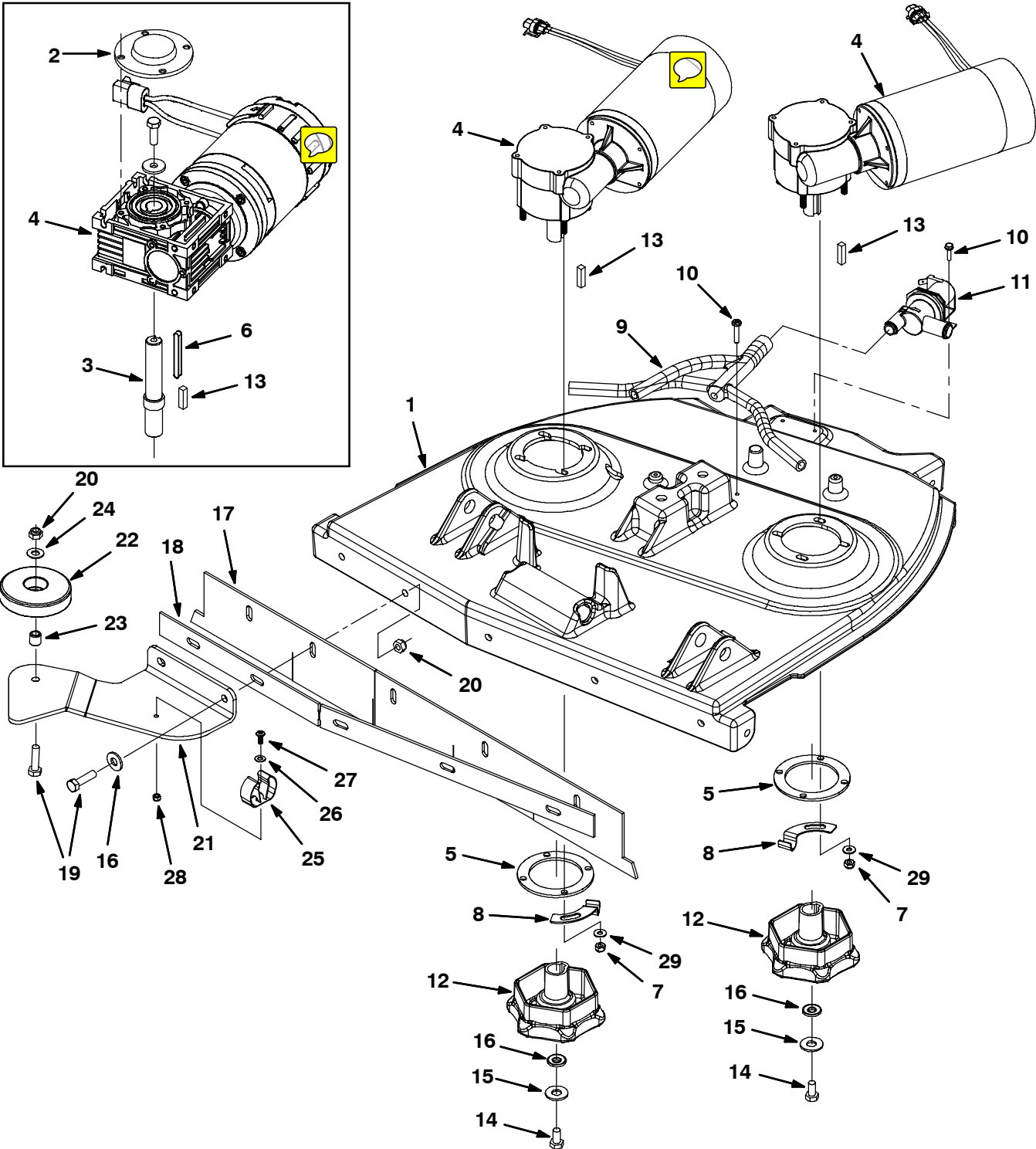
Fig. 13 - Disk Scrub Head Drive Motor Group, 650 mm
