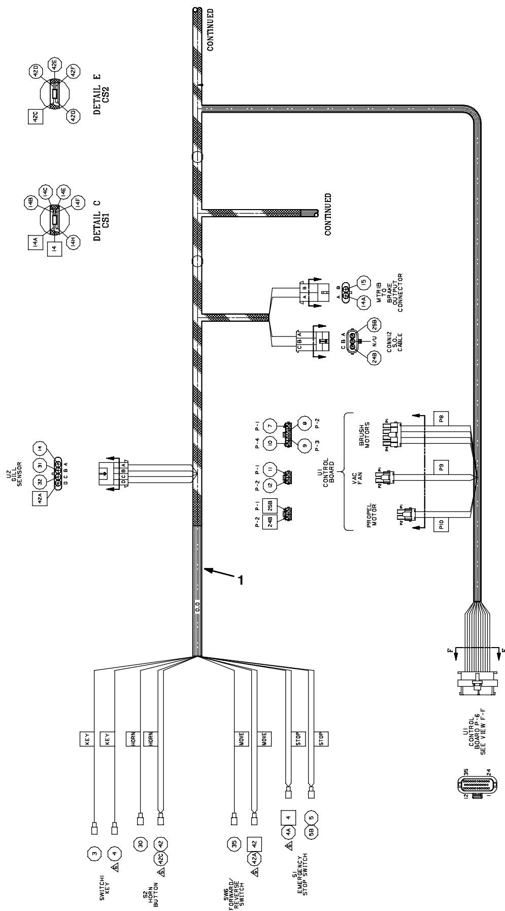
Fig. 36 - Wire Harnesses Group, Main (S/N 00000-00386)
