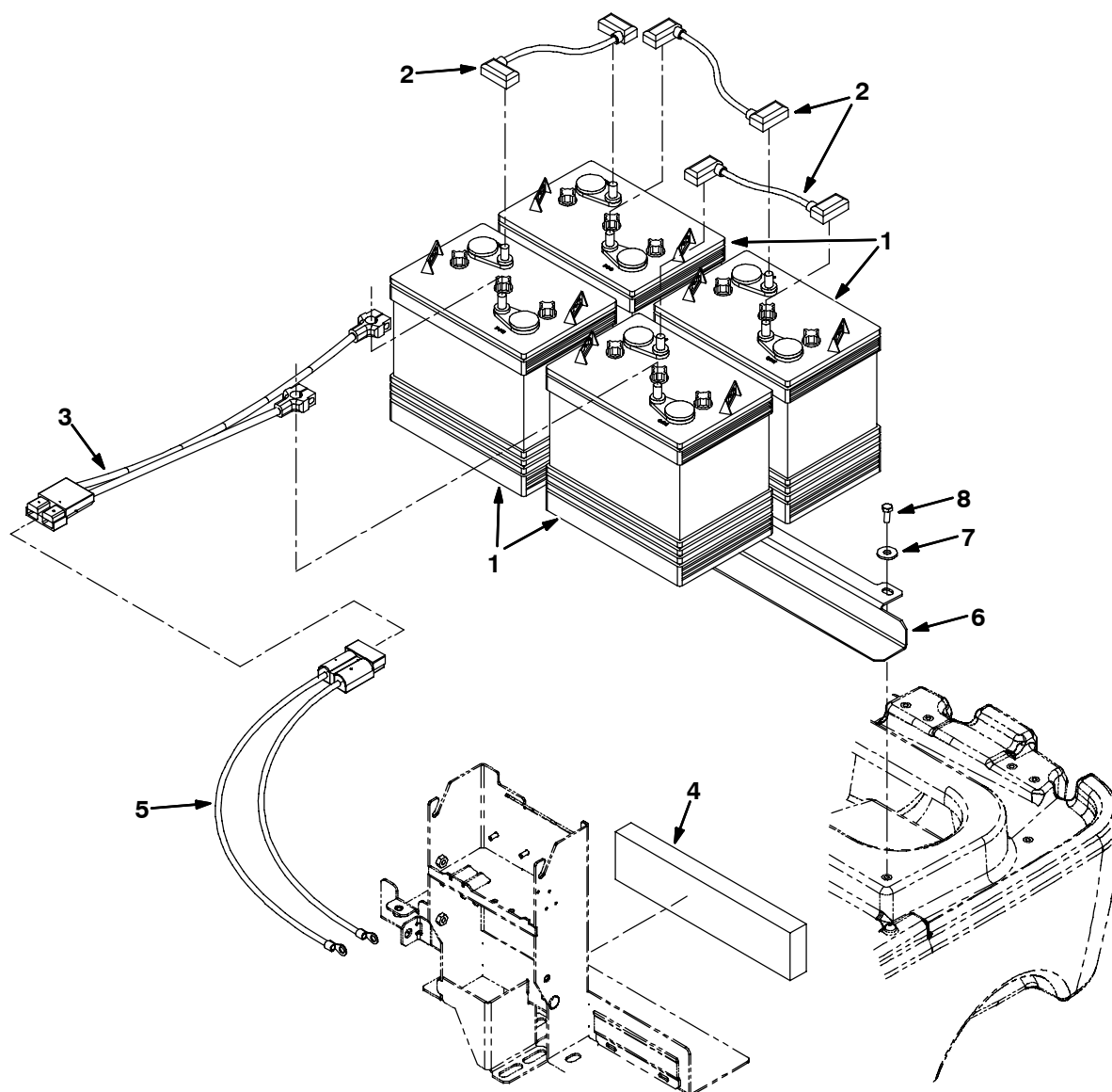
Fig. 7 - Battery and Charger Group 240Ah/5H
