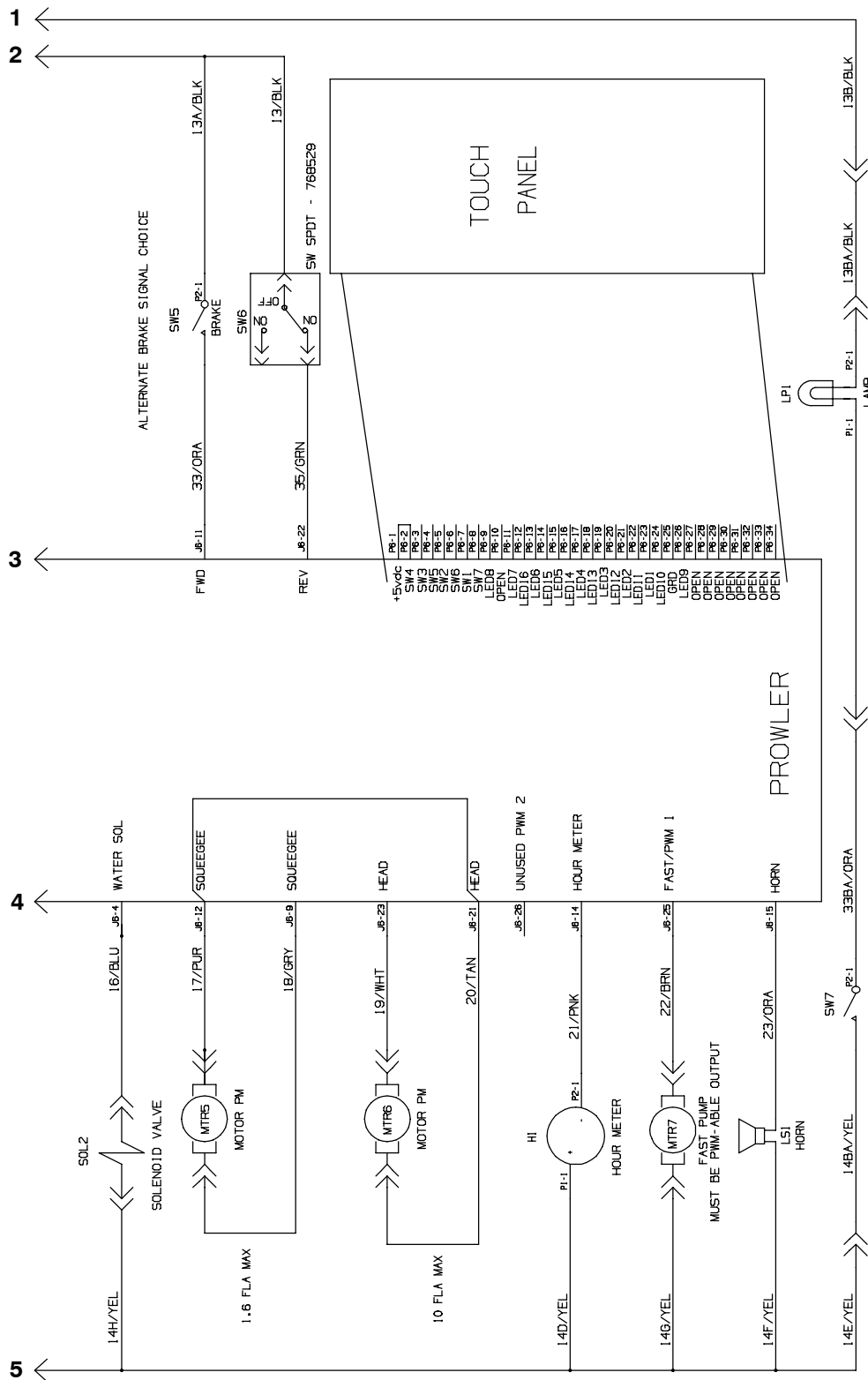
Fig. 34 - Electrical Schematic, Standard &amp; FaST Model (S/N 03000-03499)
