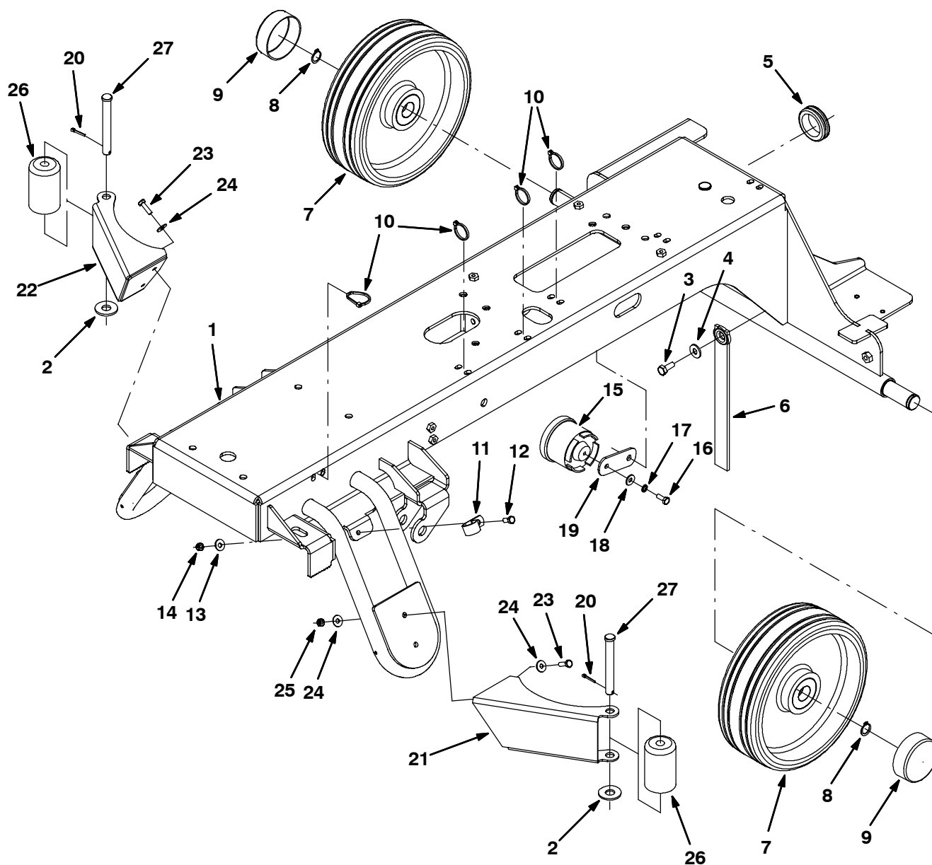
Fig. 5 - Main Frame Group, Cylindrical Scrub Head, 800 mm (32 in) (S/N 03941- )
