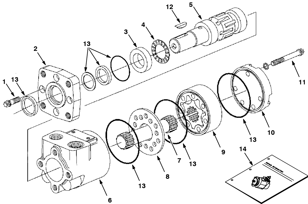
Fig. 7 - Hydraulic Motor Breakdown, 369816 - Hydraulik-Motor-Defekt - Panne de moteur hydraulique, 369816
