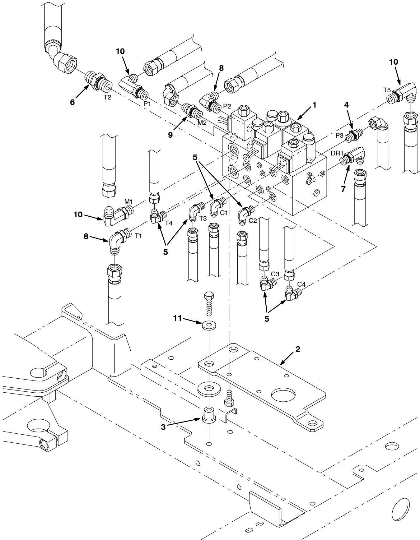
Fig. 37 - Hydraulic Valve Group - Hydraulik-Ventilgruppe - Assemblage soupape hydraulique
