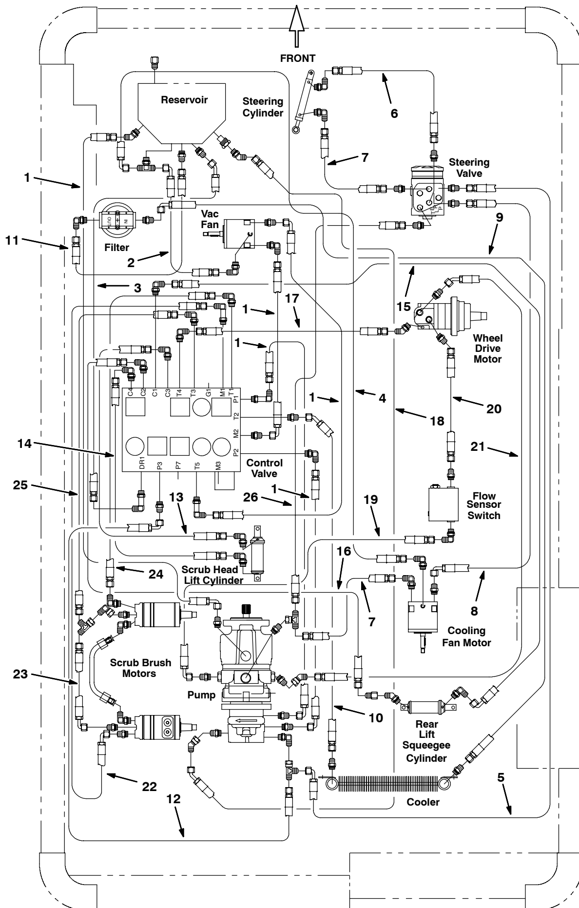
Fig. 35 - Hydraulic Hose Group - Hydraulik-Schlauchgruppe - Assemblage tuyaux hydrauliques
