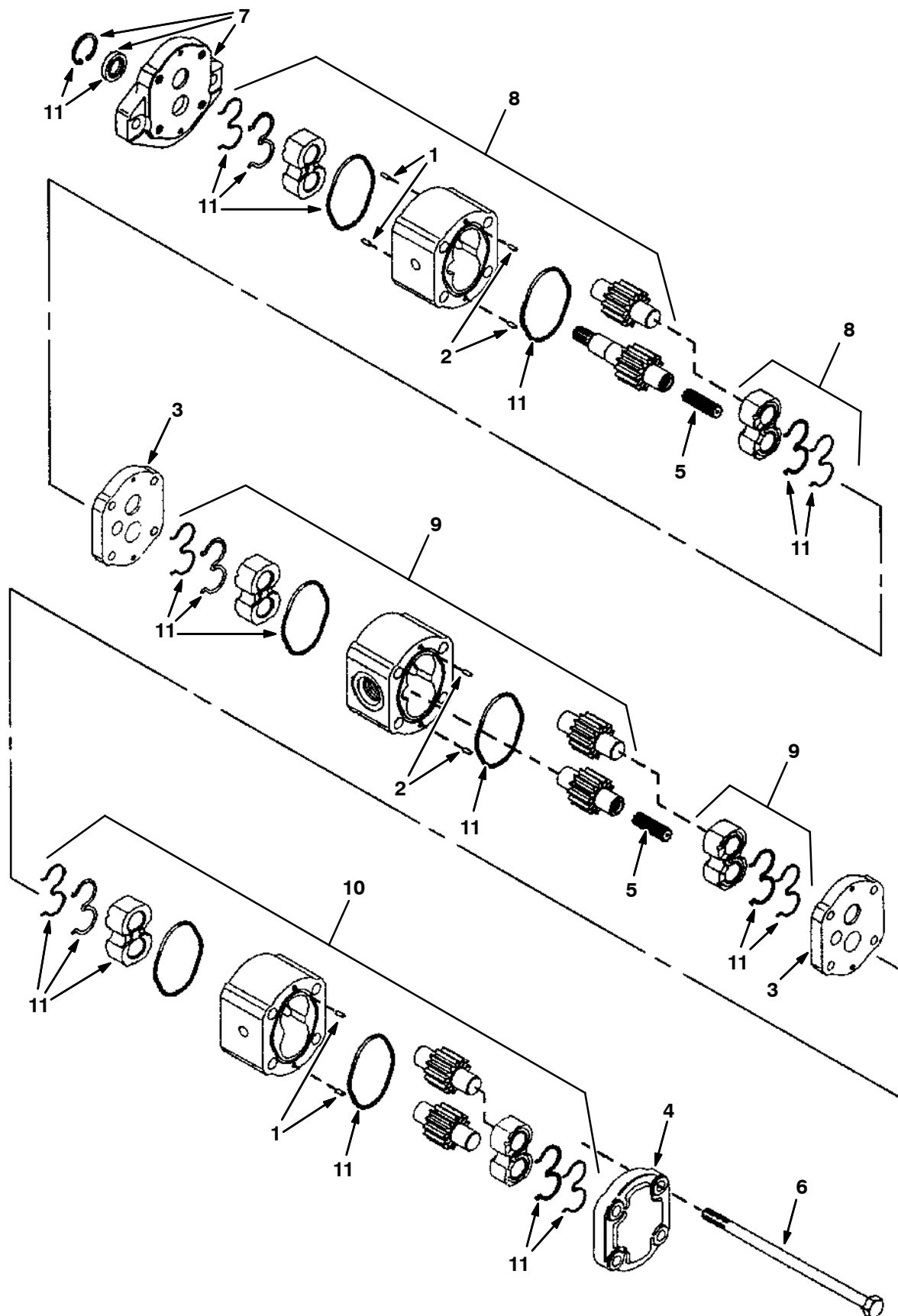
Fig. 2 - Hydraulic Pump Breakdown, 71716 - Hydraulik-Pumpen-Defekt - Panne de pompe hydraulique, 71716
