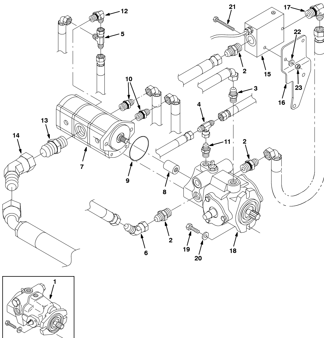
Fig. 36 - Hydraulic Pumps Group - Hydraulik-Pumpengruppe - Assemblage pompes hydrauliques
