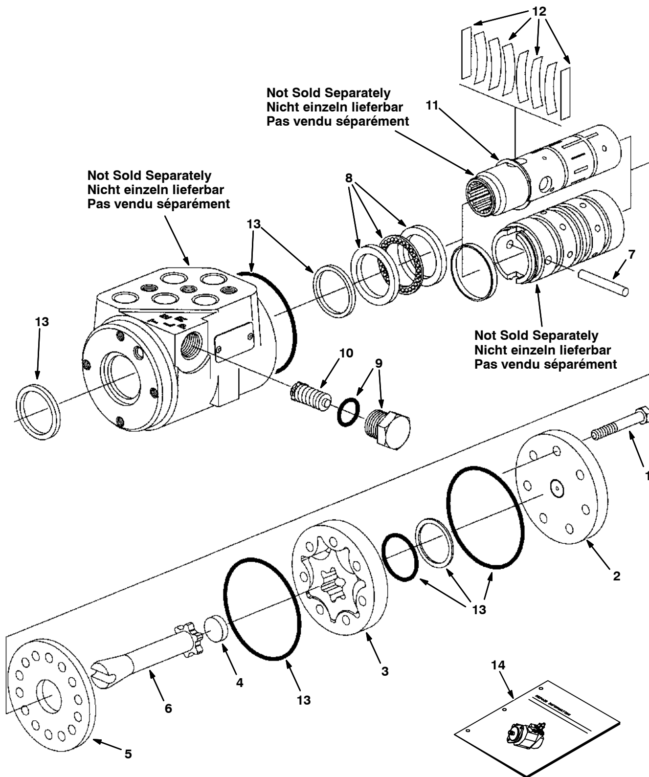
Fig. 11 - Hydraulic Steering Valve Breakdown, 71713 - Hydraulik-Lenkventil-Defekt - Panne de soupape de direction hydraulique, 71713
