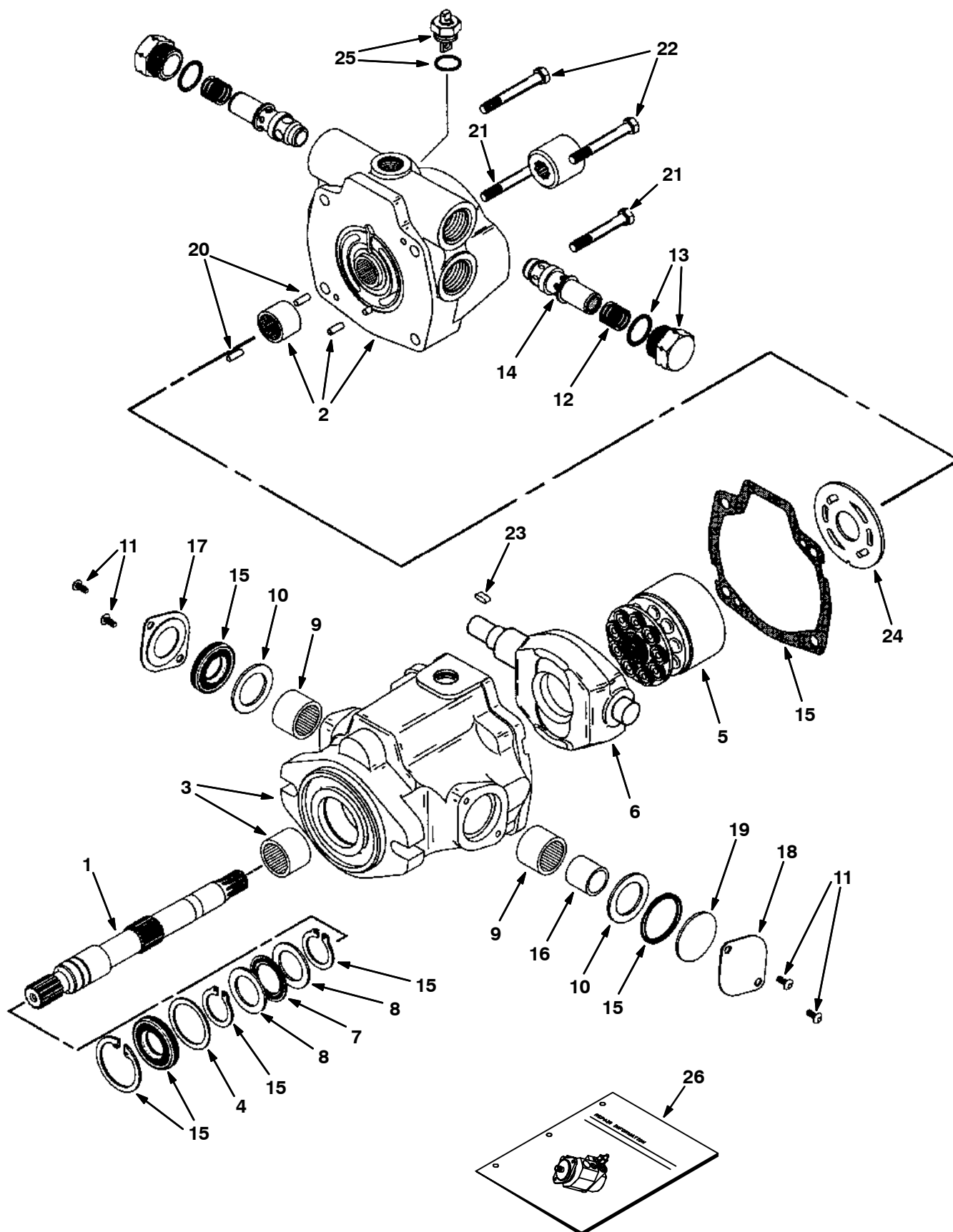
Fig. 1 - Hydraulic Pumps Breakdown, 71720 - Hydraulik-Pumpen-Defekt - Panne de pompes hydrauliques, 71720
