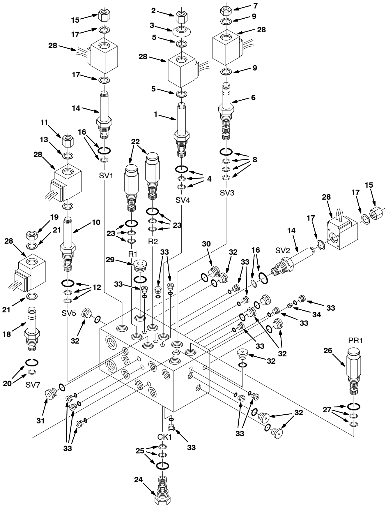
Fig. 14 - Hydraulic Solenoid Valve Breakdown, Nylon Brush, 71761 - Hydraulik-Magnetventil-Defekt, Nylon-Bürste - Panne de soupape magnétique hydraulique, brosse en nylon, 71761
