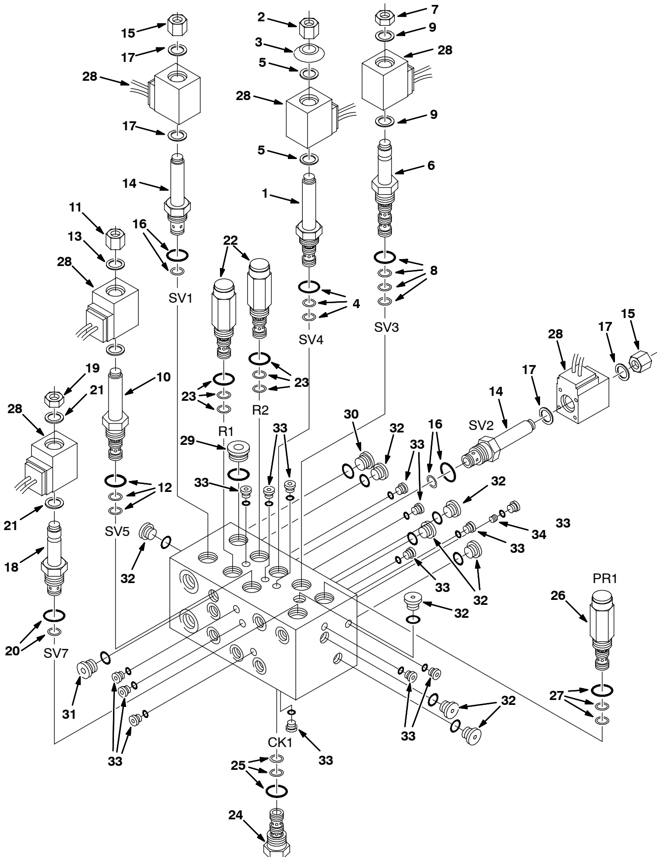
Fig. 12 - Hydraulic Solenoid Valve Breakdown, 71705 - Hydraulik-Magnetventil-Defekt - Panne de soupape magnétique hydraulique, 71705
