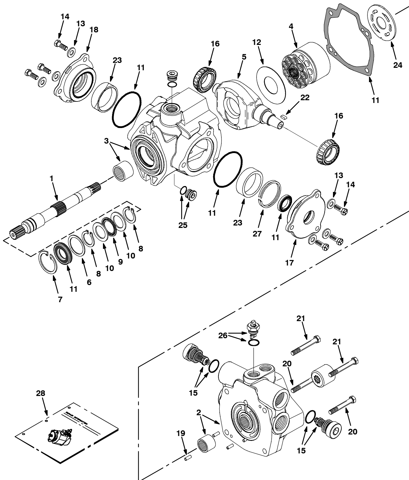
Fig. 23 - Hydraulic Pump Breakdown, 373453 - Hydraulik-Pumpen-Defekt - Panne de pompe hydraulique, 373453
